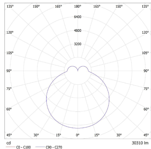
Lucis IR.L12.1500M.1 IZAR R MAX LED / LDC (Polar)
